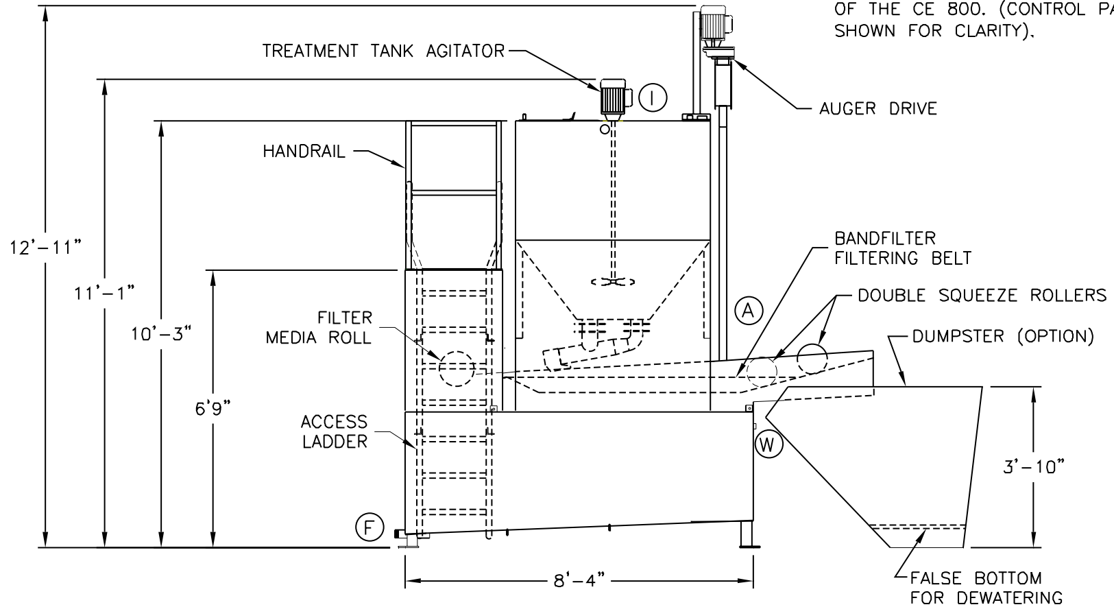
CE 800 ELEVATION DRAWING
